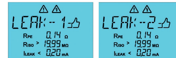
Fig. 23: Measurement of the protective conductor current on both sides
