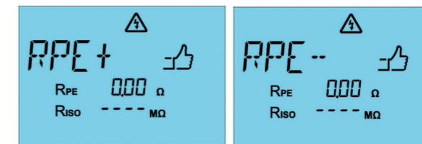
Fig. 39: R_{PE+} positive current direction (left) and R_{PE-} negative current direction (right)
