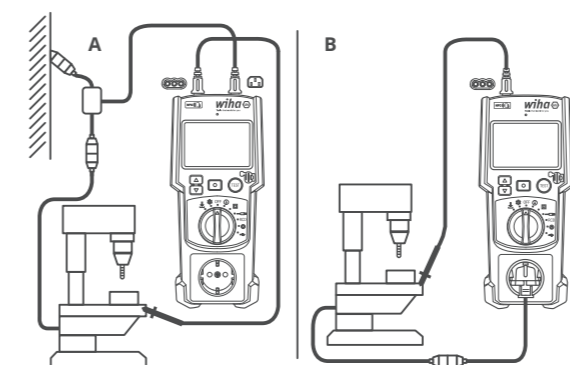
Fig. 55: Connecting the test object to the measuring device
