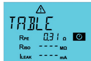
Fig. 16: Measurement interrupted; check measured value and continue or abort if necessary
