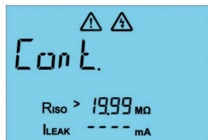
Fig. 34: Continuous measurement (cont. mode)
